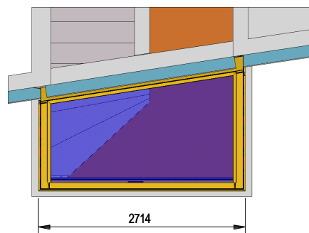
Detail W (1:50)
