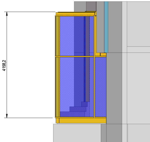
Detail V (1:50)
